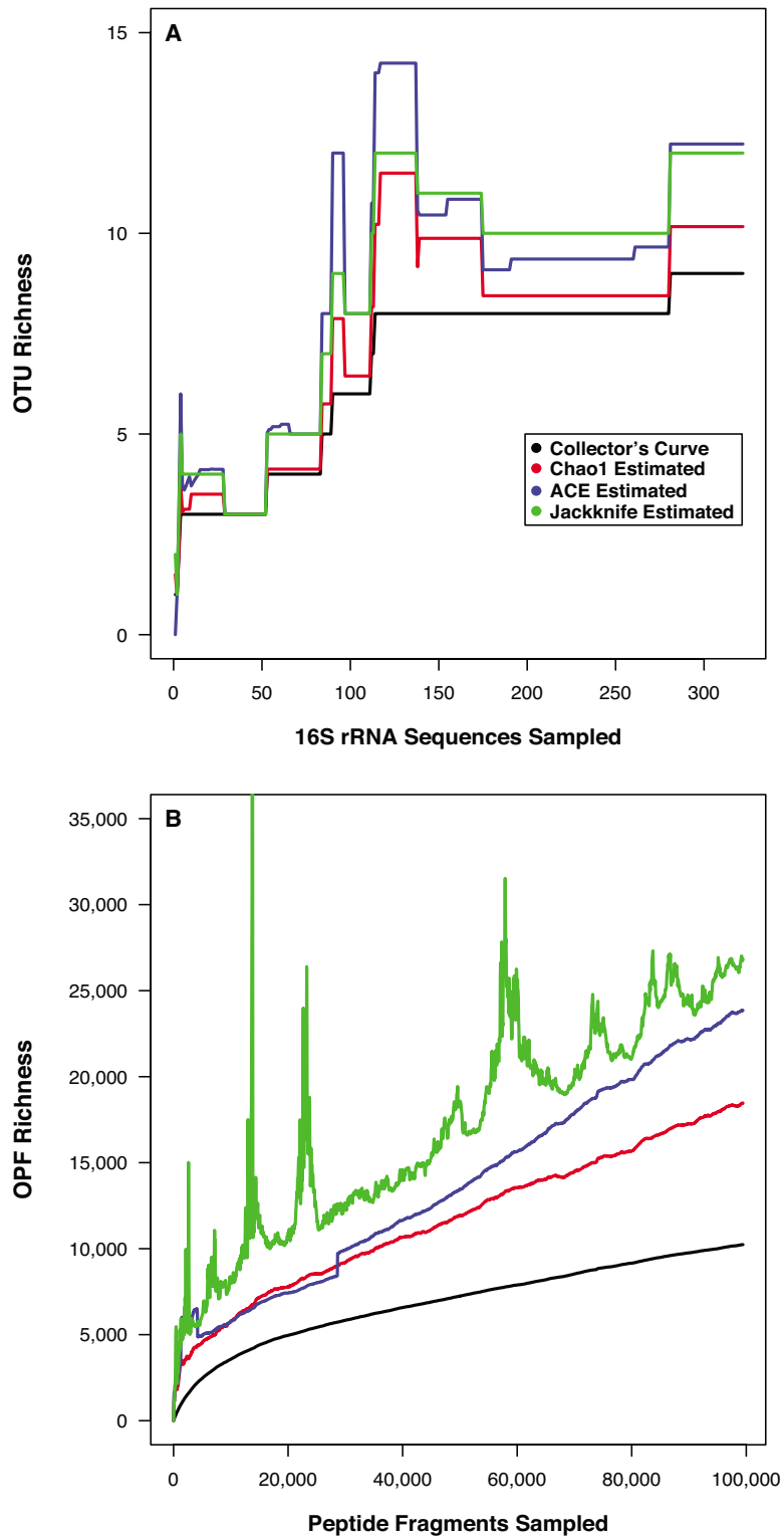
Figure 2 Collector's curves for the OTU (A) and OPF (B) richness observed and estimated using DNA extracted from an AMD biofilm community.
