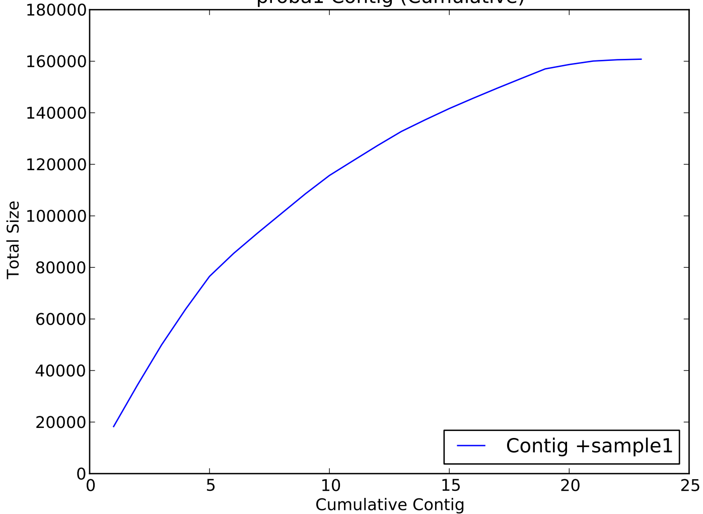
proba1 Contig (Cumulative)
